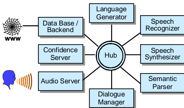
Figure 1. Block diagram of the functional components that comprise the CU Communicator system.
